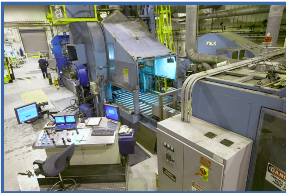
Four-High Rolling Mill With 5,000,000 Pounds of Separating Force
